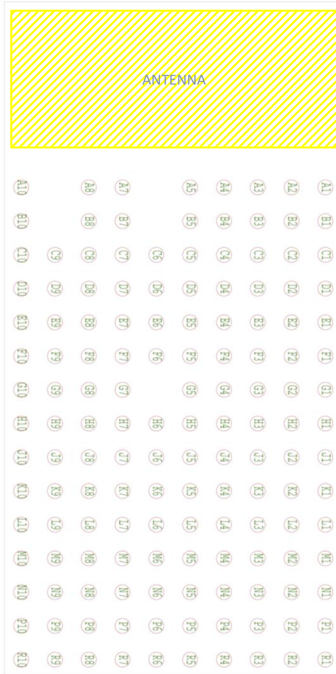
AW-CU544-PSoC62 Top View Pin Map
